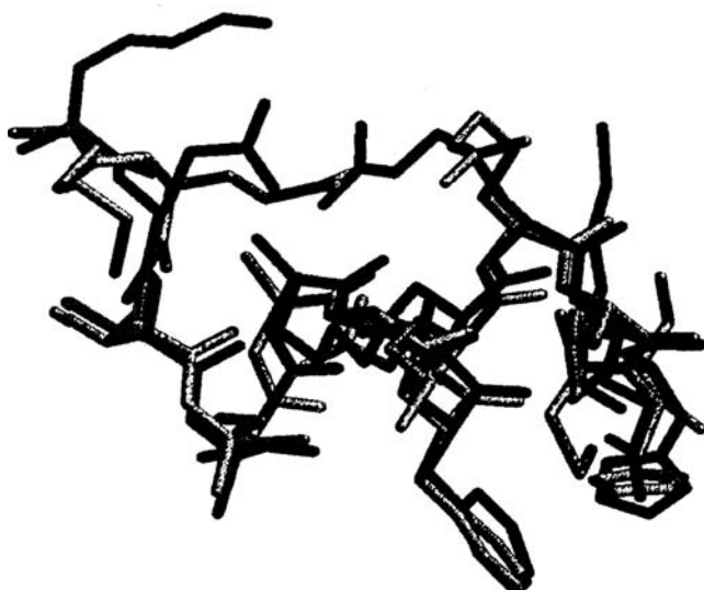
Fig. 14.2 Structure of the C-peptide of ribonuclease A: (black sticks) lowest energy state obtained from a multicanonical Monte Carlo study; (gray sticks) the X-ray structure. (After Hansmann and Okamoto, 1999.)
