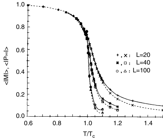
Fig. 5.2 Magnetization ( \text{—} ) and percolation probability ( \text{-- --} ) plotted vs. reduced temperature for L \times L Ising models studied using the Swendsen–Wang algorithm. After De Meo et al. (1990).
