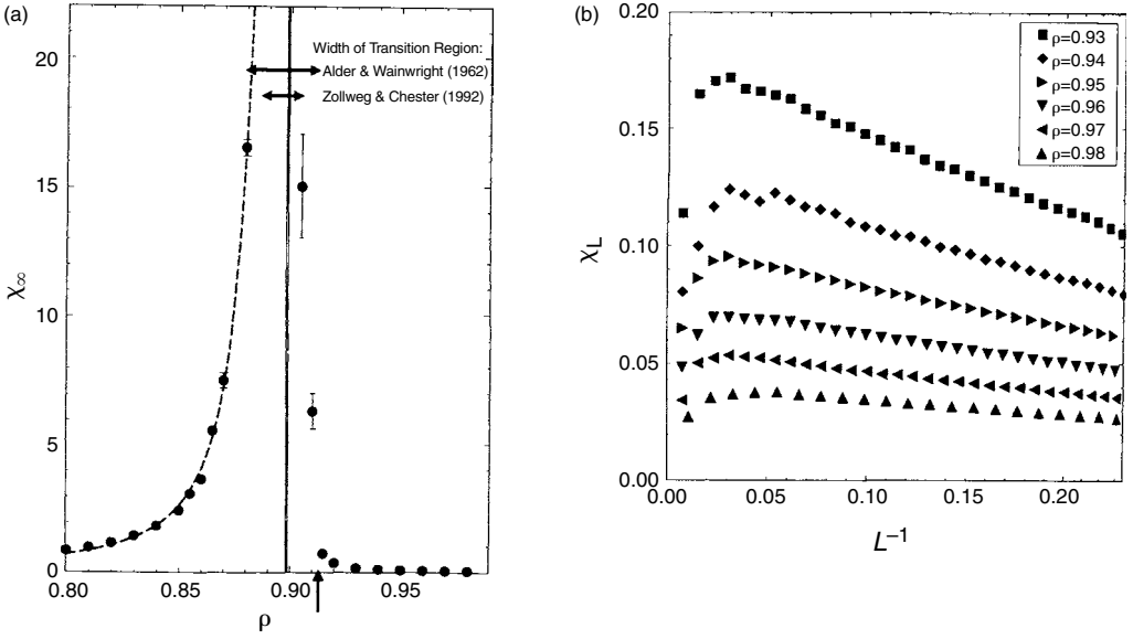
Fig. 6.6 (a) Extrapolated ‘susceptibility’ \chi_\infty of the hard disk system versus density. The data in the fluid are fitted to \chi_\infty \propto \exp\{b'(\rho_f - \rho)^{-1/2}\} where b' is a constant and \rho_f = 0.913 is marked with an arrow. The vertical solid line marks the estimated transition density \rho_{\text{cross}} = 0.8985 \pm 0.0005 obtained from cumulant intersections (Fig. 6.7). Previous estimates for the width of the two-phase region are indicated by horizontal arrows. Error bars are only shown when they exceeded the size of the symbols. (b) Susceptibility \chi_L as a function of the inverse linear subsystem size L^{-1} in the solid phase away from the transition, for N = 16\,384 particles. From Weber et al. (1995).
