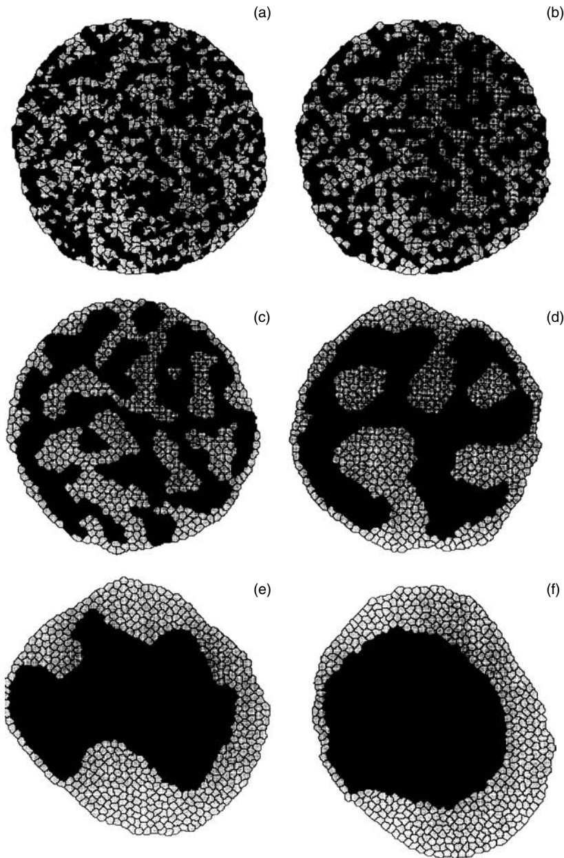
Fig. 13.4 Time dependence of cell sorting for two different cell types: (a) initial, randomly assigned cell type; (b) 1 MCS; (c) 100 MCS; (d) 1000 MCS; (e) 4000 MCS; (f) 10 000 MCS. From Graner and Glazier (1992).
