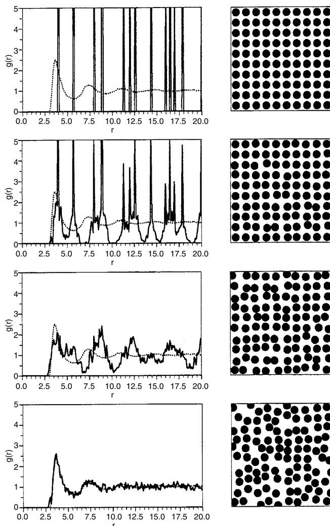
Fig. 5.17 Application of the reverse Monte Carlo method to a two-dimensional Lennard-Jones system. On the left is the development of the radial distribution function. The dotted curves give the target ‘data’ (obtained by the Metropolis method) and the solid curves show the instantaneous distributions obtained from intermediate particle configurations (shown on the right). After McGreevy (2001).
