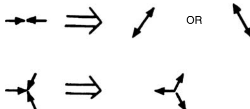
Fig. 12.6 Lattice gas cellular automata collision rules for particle movement on a triangular lattice.
