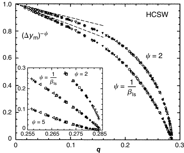
Fig. 6.3 Scaling plots for the HCSW fluid. Note that \Delta y_m and q are related to the difference in the scaling variable for the mean density and the 4th order cumulant, respectively. (After Kim, Fisher, and Luijten, 2003.)
