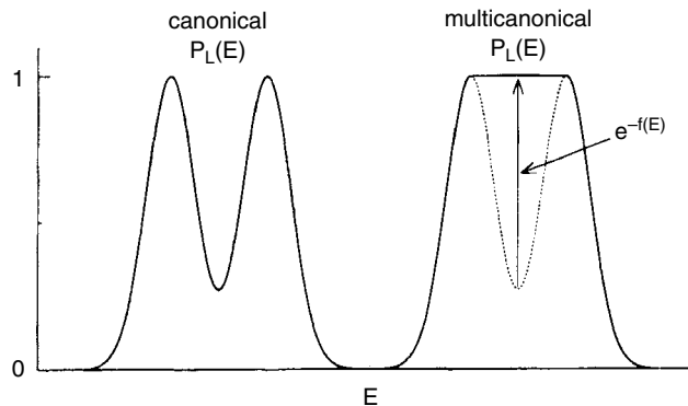
Fig. 7.4 Probability distribution for canonical Monte Carlo sampling for a model with multiple minima compared to that for multicanonical Monte Carlo.
