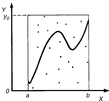
Fig. 3.1 Simple representation of 'hit-or-miss' Monte Carlo integration of a function f(x) , given by the solid curve, between x = a and x = b . N points are randomly dropped into the box, N_o of them fall below the curve. The integral is estimated using Eqn. (3.2).
