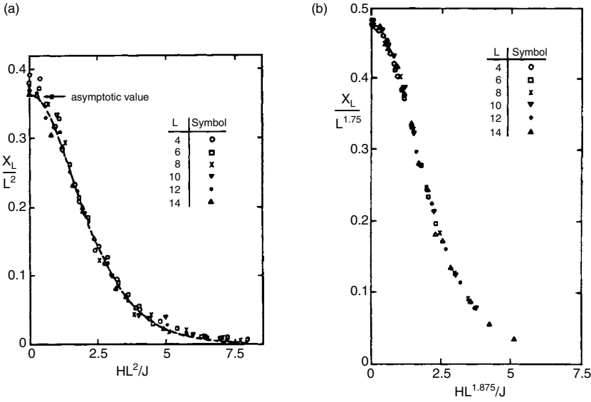
Fig. 4.7 Finite size scaled susceptibility vs. scaled field for the two-dimensional Ising model along paths of constant temperature: (a) k_B T / J = 2.1 ; (b) k_B T / J = 2.269 = T_c . From Binder and Landau (1984).
