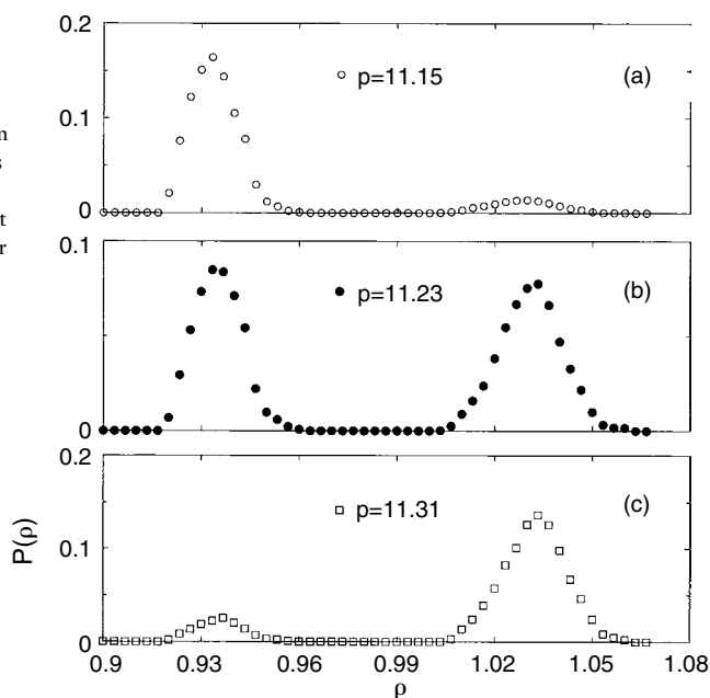
Fig. 6.10 The distribution of the density of the system of N = 256 particles at pressures (a) just below; (b) at; (c) just above coexistence for this N . The mean single phase density averages are \rho_F = 0.934(3) and \rho_{CS} = 1.031(4) .
