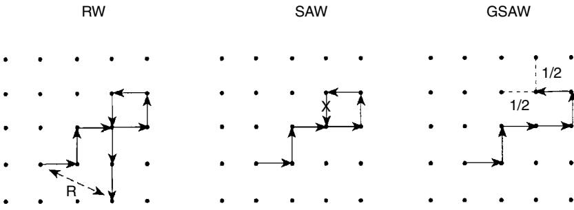
Fig. 3.6 Examples of different kinds of random walks on a square lattice. For the RW every possible new step has the same probability. For the SAW the walk dies if it touches itself. The GSAW walker recognizes the danger and takes either of the two steps shown with equal probability.
