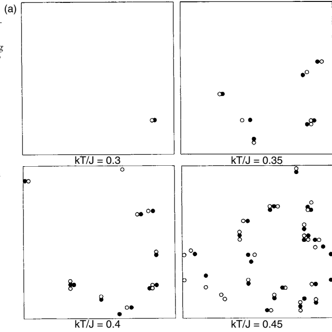
Fig. 5.7 Topological (a) excitations in the two-dimensional anisotropic Heisenberg model. (a) 'Snapshots' of vortex behavior in the SF state for L = 40, H_{\parallel}/J = 4.0 . Open and closed circles represent vortices and antivortices, respectively. (b) Vortex-pair density in the SF state. The energy (in units of J ) needed to create a vortex-antivortex pair is 2\mu . From Landau and Binder (1981).
