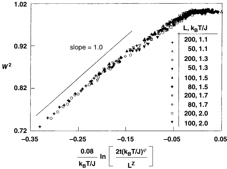
Fig. 10.12 Dynamic finite size scaling of the surface width for 2 + 1 dimensional MBE models. The growth exponent \beta = 0 and the dynamic exponent z = 1.63 for this plot. From Pal and Landau (1999).
