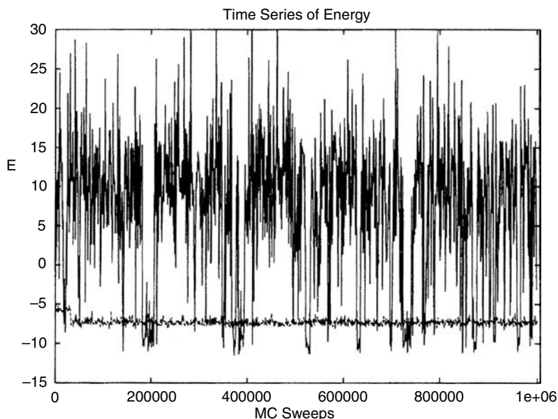
Fig. 14.1 Time sequence of the energy of simulations for Met-enkephalin from a regular canonical simulation at T = 50 K (dotted curve) and from a generalized ensemble simulation (solid curve). (After Hansmann and Okamoto, 1999.)
