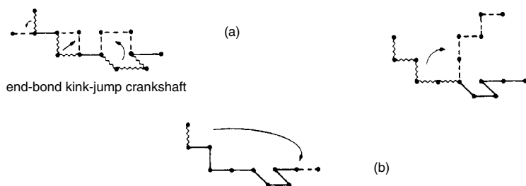
Fig. 4.26 Dynamic Monte Carlo algorithms for SAWs on a simple cubic lattice: (a) generalized Verdieer-Stockmayer algorithm; (b) slithering snake algorithm; (c) pivot algorithm.
