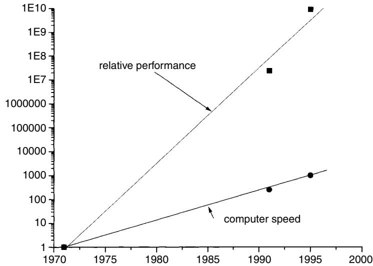
Fig. 5.18 Approximate variation of Ising model simulation performance with time: (upper curve) total relative performance; (lower curve) relative improvement in computer speed.
