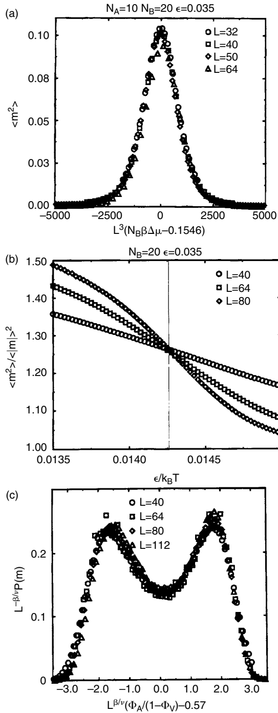
Fig. 6.18 Data for asymmetric polymer mixtures. Scaling of the second moment of the order parameter at \epsilon/k_B T = 0.035 (a); locating the critical temperature from the intersection of moment ratios (b); scaled order parameter distribution at criticality (c). In all cases the different symbols indicate different linear dimensions L .
