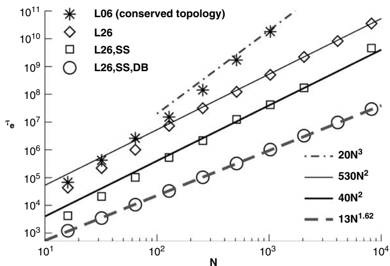
Fig. 6.21 Log-log plot of relaxation time \tau_e (defined from the time needed for a chain to diffuse over its end-to-end distance) vs. chain length N for different algorithms for the bond fluctuation model at a volume fraction \phi = 0.5 . Asterisks denote the L06 algorithm, diamonds the L26 algorithm, squares the algorithm (where L26 and SS moves are randomly mixed), and circles show the algorithm where DB moves are also included (see the text). Straight lines show fits to power laws \tau_e \propto N^3 (dash-dotted), \tau_e \propto N^2 (full lines), and \tau_e \propto N^{1.62} (broken line). From Wittmer et al. (2007).
